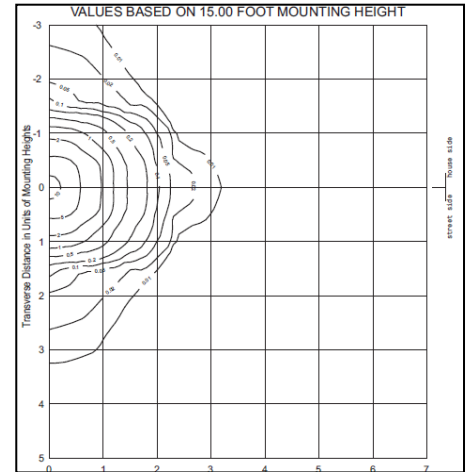
IES Road Report Isolines (Type III)
